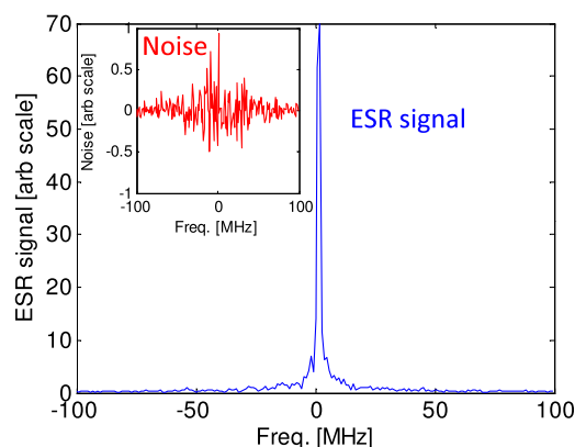
FIG. 2. ESR signal and noise in the spectral domain for the ^{28}\text{Si}:\text{P} sample at 10 K, around a center frequency of 34.1 GHz using a MW peak power of 0.2 mW. For signal acquisition, we employed a Carr-Purcell-Meiboom-Gill (CPMG) pulse sequence with a repetition rate of 600 Hz, \pi/2 pulse length of 30 ns, \pi/2\text{-}\pi pulse separation, \tau = 1.2\ \mu\text{s} , and a data acquisition window of 1\ \mu\text{s} . Data are averaged from shot to shot and also along each of the 160- \pi -pulse CPMG echo trains, resulting in overall 600 \times 160 = 96\,000 averages in 1 s.
